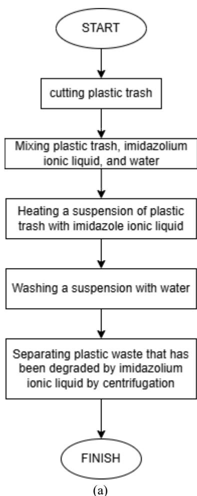
Fig. 4. (a) Flowchart of the processing plastic trash using Imidazolium Ionic Liquid, (b) the combustion process utilizing the incinerator
