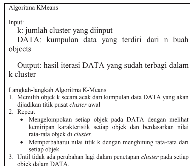
Gambar 1 Algoritma KMeans [2]
