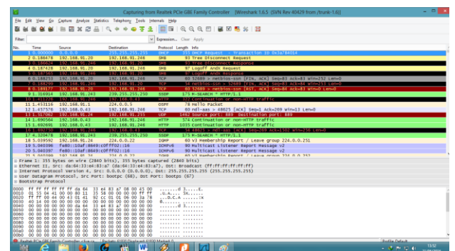
Gambar 9. Tampilan Wireshark
