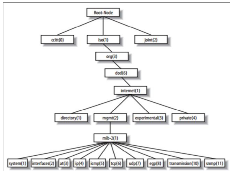
Gambar 1. MIB Tree
