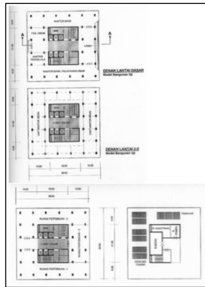
Gambar 2: Denah model bangunan uji lt.dasar – lt.atap
